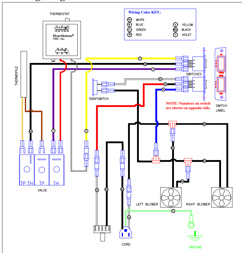
Figure 7 Wiring Diagram
